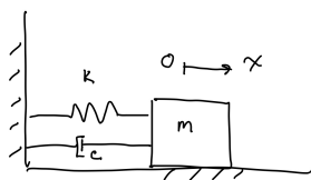
(a) A single degree of freedom harmonic oscillator, or SDOFHO for confusing and short.
